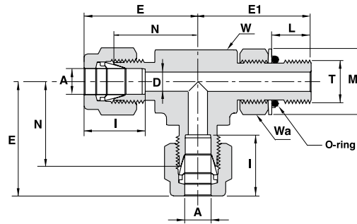
TUBE TO SAE/MS STRAIGHT THREAD BOSS (POSITIONABLE)*
