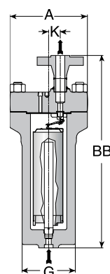
Series 6000 FW Trap
