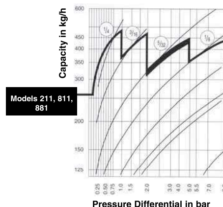
Chart ST-77-1: Selection Curve Example 1
