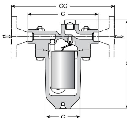
Model 421 Trap
