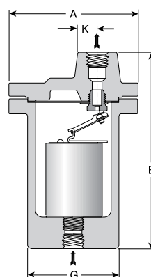
Model 300 Trap
