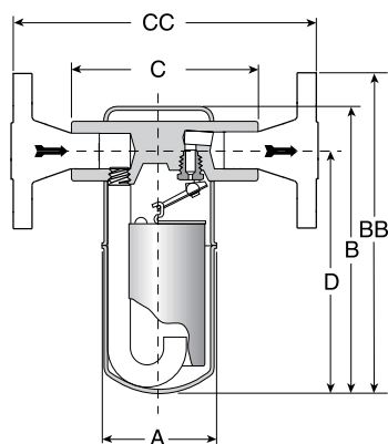
Model 1811 Trap
